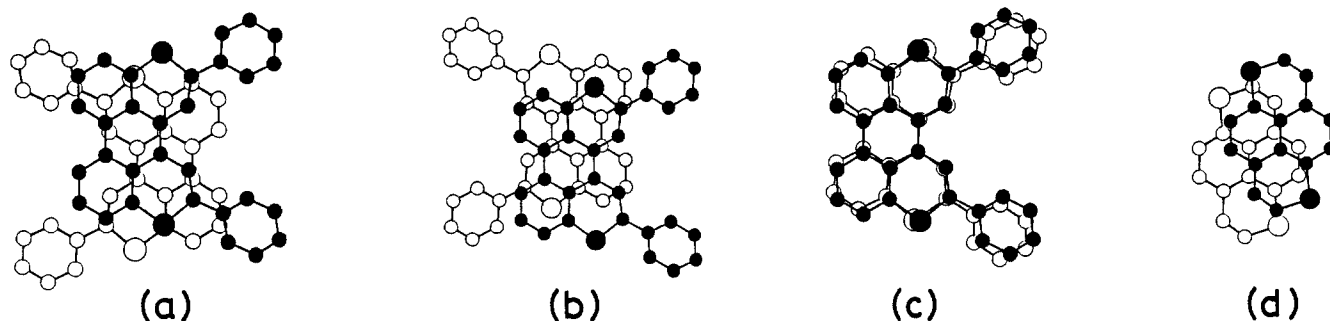
Figure 3. The modes of the molecular overlap. The view direction is perpendicular to the molecular plane: (a) the neutral \text{Ph}_2\text{DTPR} ; (b) and (c) the cation radicals of \text{Ph}_2\text{DTPR} ; (d) the neutral \text{DTPY} .
