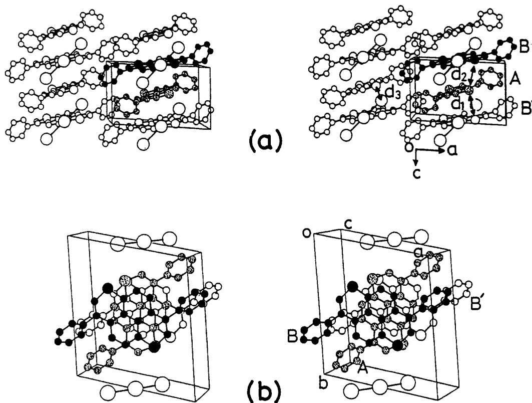
Figure 7. Stereoviews of the crystal packing for (Ph 2 DTPY) 2 -I 3 . The view directions are (a) along the b axis and (b) normal to the DTPY skeleton of the molecule A.
