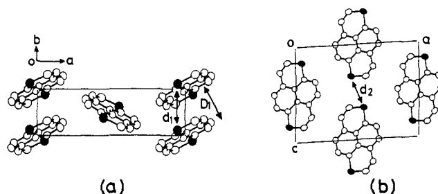
Figure 6. Crystal structures of the neutral DTPY: (a) view along the c axis and (b) view along the b axis.
