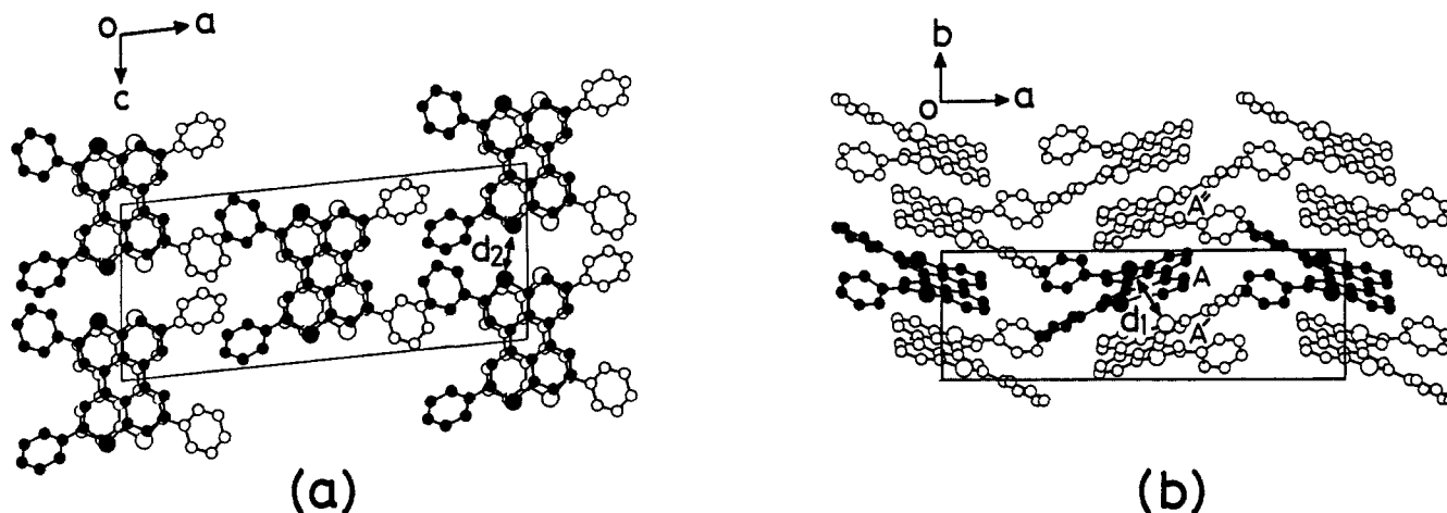
Figure 2. Crystal structures of \text{Ph}_2\text{DTPR} viewed along (a) the b axis and (b) the c axis.
