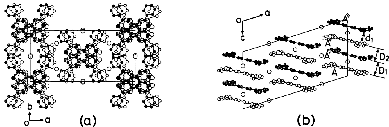
Figure 4. Crystal structures of \text{Ph}_2\text{DTPR-ClO}_4 viewed along (a) the c axis and (b) the b axis. The symmetry operations are the following: A(x, y, z) , A'(2-x, y, 1.5-z) , A''(x, -y, -0.5+z) , A'''(2-x, -y, 1-z) .
