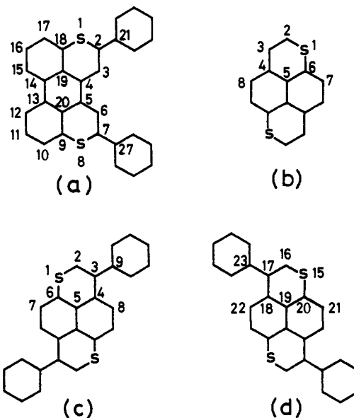
Figure 8. The atomic numbering schemes for (a) \text{Ph}_2\text{DTPR} , (b) \text{DTPY} , (c) the molecule A of (\text{Ph}_2\text{DTPY})_2\text{-I}_3 , and (d) the molecule B of (\text{Ph}_2\text{DTPY})_2\text{-I}_3 .
