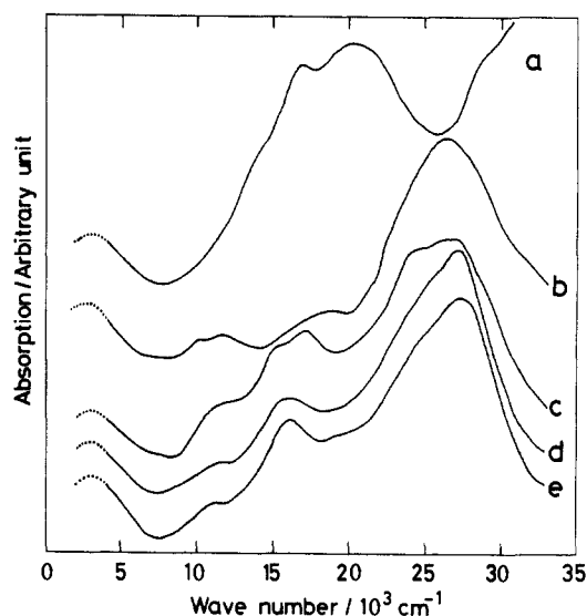
Figure 1. Absorption spectra of (a) Ph 2 DTPR-DDQ 0.75 , (b) TTF-TCNQ, (c) DTPY-TCNQ, (d) DTPY-THBTCNQ, and (e) DTPY-DHBTCNQ as powders dispersed in KBr.
