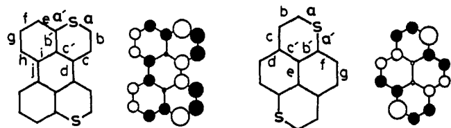
Figure 5. Numbering scheme for bond lengths and highest occupied molecular orbitals of DTPR and DTPY.
